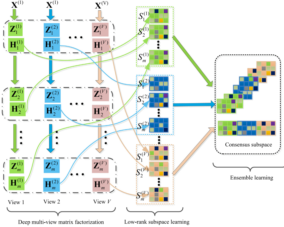
Fig. 17. The framework of deep Low-Rank Subspace Ensemble (DLRSE) method for multi-view clustering (adapted from [17]).
