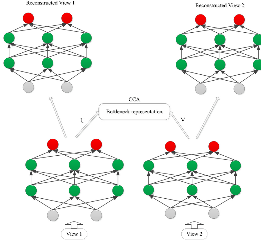
Fig. 13. The framework of deep canonical correlated auto-encoders (DCCAE) (adapted from [22]).
